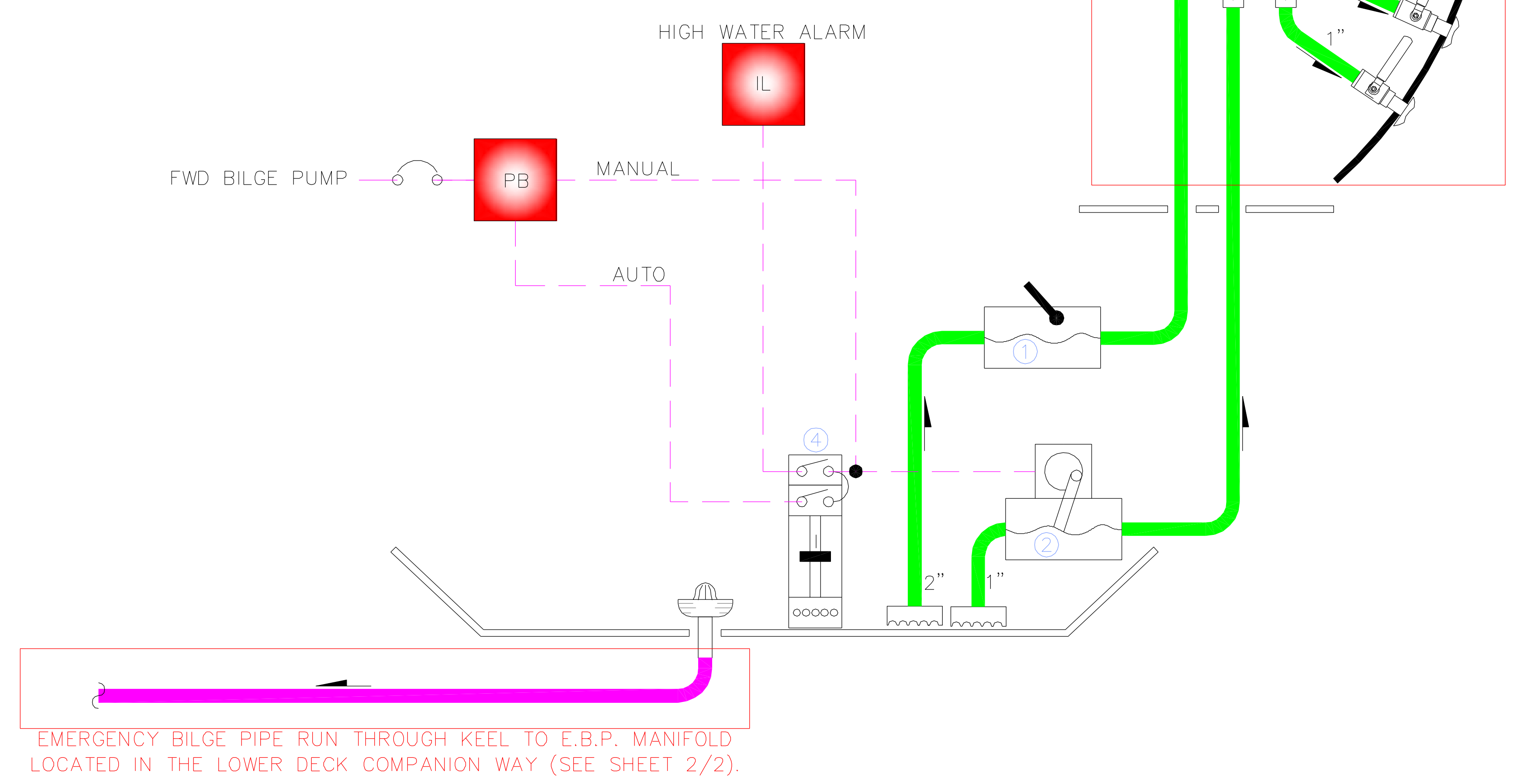
FWD BILGE COMPARTMENT (BELOW LOWER DECK COMPANION WAY)
