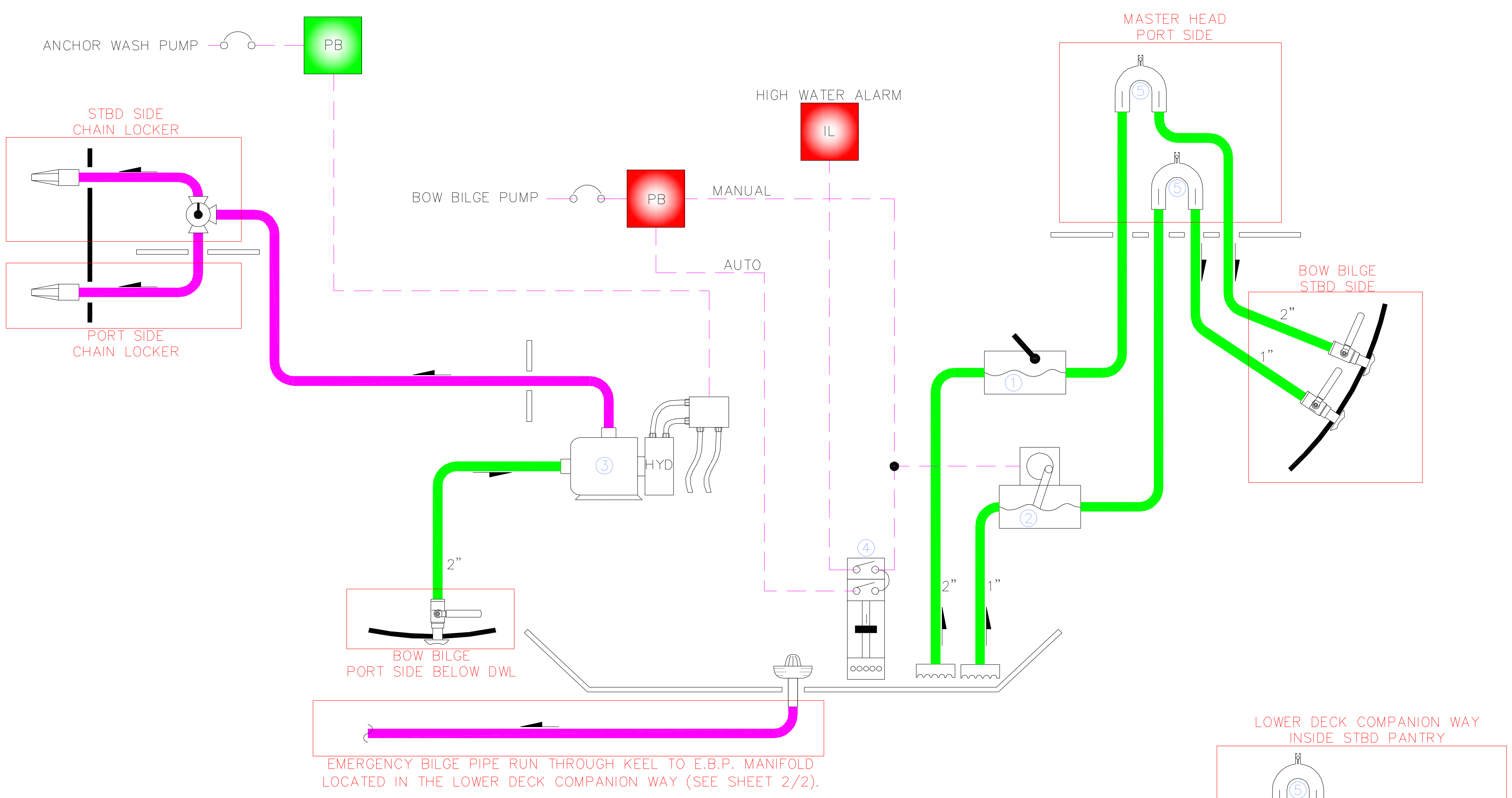
BOW BILGE COMPARTMENT (BELOW MASTER STATEROOM HEAD)
