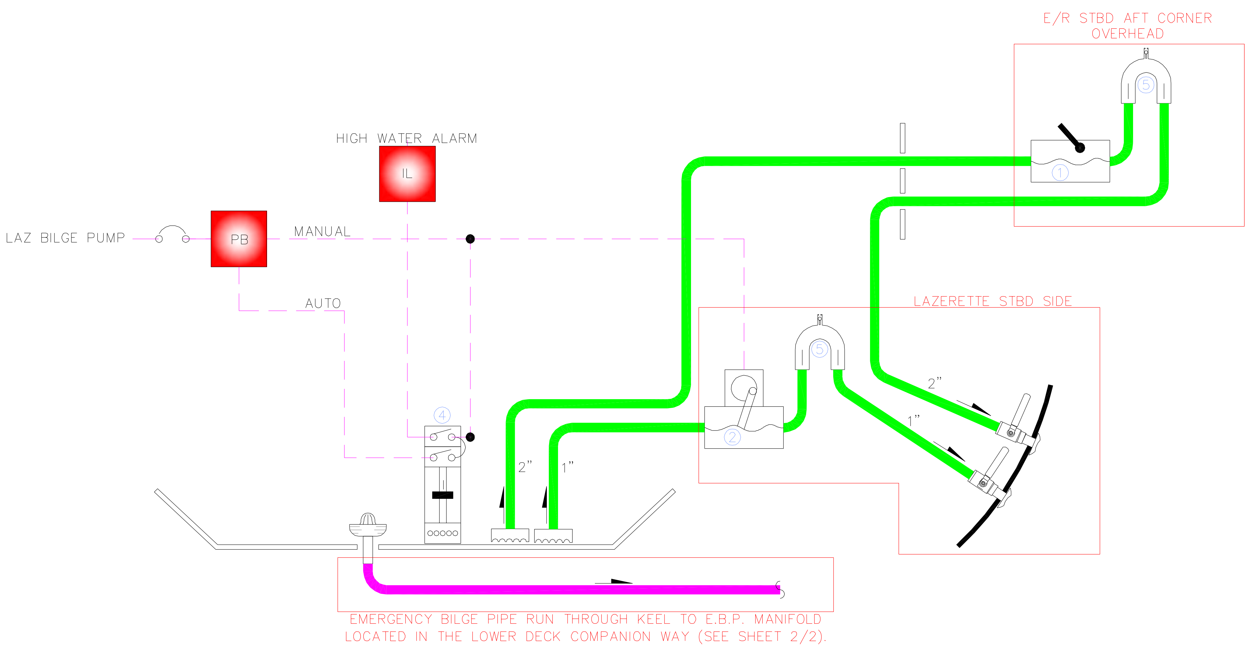
LAZ BILGE COMPARTMENT (BELOW LAZERETTE FWD DECK PLATE)
