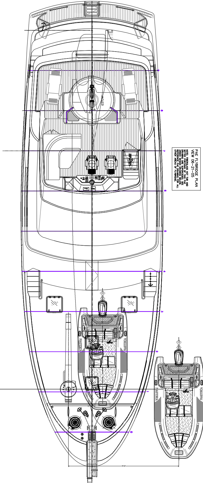
ARDEO DESIGN FLYBRIDGE PLAN VIEW 06-22-05
