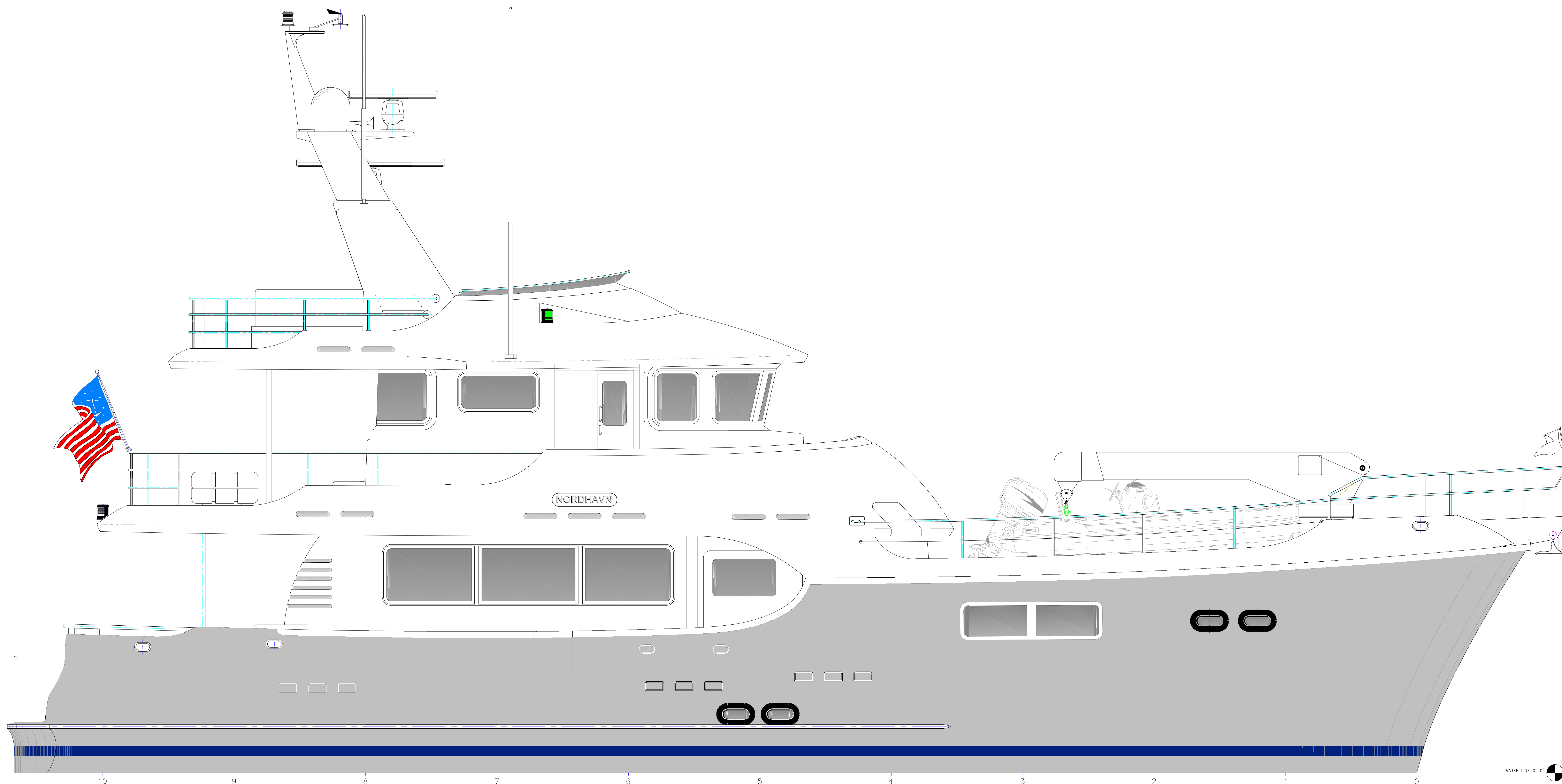
STARBOARD PROFILE 1/2"=1'-0"
